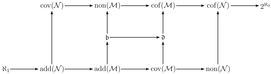
Fig. 1 Cichoń’s diagram. An arrow between \aleph and \eta indicates that \aleph \leq \eta . Moreover, \max(\mathfrak{d}, \text{non}(\mathcal{M})) = \text{cof}(\mathcal{M}) and \min(\mathfrak{b}, \text{cov}(\mathcal{M})) = \text{add}(\mathcal{M})
