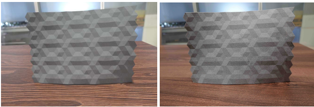
Fig. 31. A smooth surface was roughened via vertex displacements along vertex normals, v_i^f = v_i + 0.1 n_i , following a regular 3D texture. The resulting mesh had a maximum dihedral angle \max_e \alpha_e = 16.4^\circ . It was subsequently optimized with \alpha_e^{\max} = 10^\circ for all e \in E . The texture used in the initialization is clearly visible in the result, \mathcal{R} = 0.075 . Remarkably, our rendering (left) closely captures the visual appearance of the fabricated model (right).
