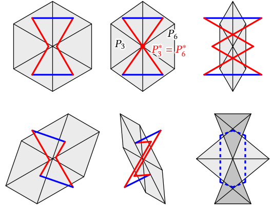
Fig. 19. Vertex stars (shaded) and their dual hexagons for a hyperbolic surface point. Different edge colors indicate angles of different signs. The top row shows principal symmetric stars. The star in the middle has four edges in asymptotic directions ( \phi = \text{atan} \sqrt{|\kappa_1/\kappa_2|} ) and thus the marked triangles are coplanar ( P_3 = P_6 ) and two vertices of the dual hexagon agree. Non-intersecting, convex hexagons can only arise from invalid vertex stars (bottom right).
