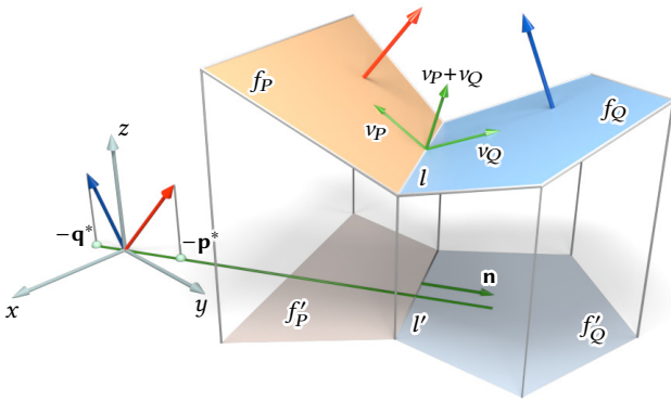
Fig. 14. Dihedral angles between two faces of a polyhedral surface in \mathbb{I}^3 can be oriented. If the sum v_P + v_Q of the two edge-normal vectors pointing to the interior of their respective faces has positive z -coordinate, we call the angle positive. The edge vector \mathbf{q}^* - \mathbf{p}^* of the dual diagram is orthogonal to the top view l' of the edge l and it is the signed angle a_s(P, Q) times the unit normal vector \mathbf{n} pointing from f'_P to f'_Q .
