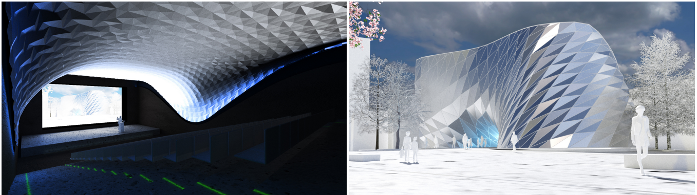
Fig. 1. Triangle meshes with controlled roughness as a design element in architectural applications. The ceiling of the auditorium has been computed from a triangulated reference surface by an automatic roughening algorithm, which creates a structured visual appearance and enables the designer to control the dihedral angles under orientation constraints. The façade is a triangle mesh whose vertices lie on a given smooth reference surface. The mesh has been created by a remeshing algorithm that locally aligns the mesh edges such that the desired level of roughness is achieved, with a smooth appearance towards the entrance, and rougher towards the right-hand side. The alignment of mesh edges depends on the local curvature behavior and is based on our thorough analysis of the relation between the local positioning of vertex stars and the visual appearance of a mesh.
