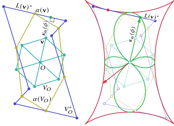
Fig. 16. Relation between the top view of a vertex star and its dual hexagon at a negatively curved point. Left : Given is a vertex star V_O with central vertex O and 1-ring vertices \mathbf{v} . The edge L(\mathbf{v})^* of the dual hexagon V_O^* is orthogonal to the corresponding edge from O to \mathbf{v} . The distance from O to L(\mathbf{v})^* is \kappa_n(\phi) . The affine map \alpha: (\xi, \eta) \mapsto \frac{1}{2}(\kappa_1\xi, \kappa_2\eta) maps the 1-ring vertices \mathbf{v} to a hexagon whose vertices \alpha(\mathbf{v}) pass through the edges of the dual hexagon. Right : The radial diagram of the normal curvature (green) with polar coordinates (\phi, \kappa_n(\phi)) is an algebraic curve of order 6. The dual edges L(\mathbf{v})^* also envelope an algebraic curve of order 6 (red).
