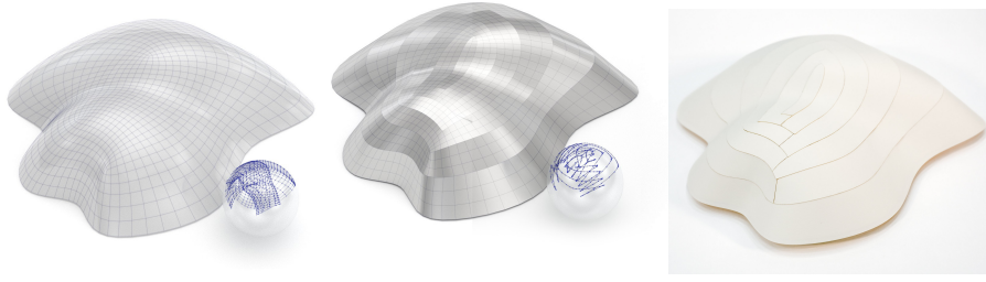
Fig. 17. The surface on the left is made piecewise developable by partitioning it into strips along mesh polylines, and making those strips developable while boundaries remain fixed. We also show the Gauss image, whose curve components correspond to the developable parts of the surface. The figure on the right shows a paper model.
