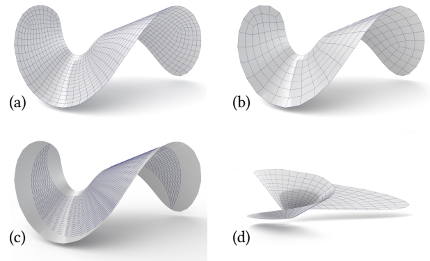
Fig. 26. Invariance of developability under remeshing and projective maps. Remeshing converts mesh (a) to meshes (b), (c), and a projective transformation yields (d). E_{dev} remains small — see Table 2.
