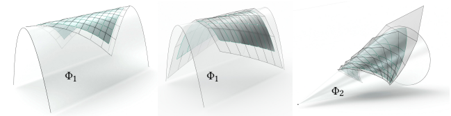
Fig. 13. A projective transformation maps the parabolic cylinder \Phi_1 to a quadratic cone \Phi_2 . \Phi_1 has many exact representations by a discrete-developable quad mesh and associated biquadratic spline surface (left and center). The projective transformation maps spline control points of \Phi_1 to weighted spline control points of \Phi_2 , leading to a quadratic NURBS representation. This low degree is possible with polynomial (un-weighted) splines only in special cases, namely, if parameter lines are rulings.
