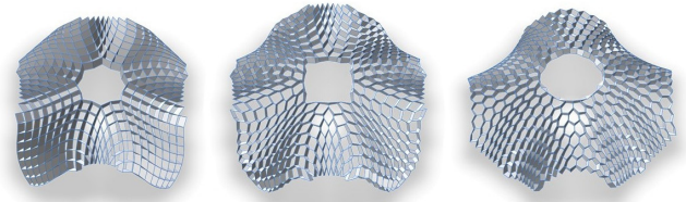
Fig. 15. Hex meshes via edge insertion. Splitting vertices in the quad-C-mesh on the left results in a hex mesh (center). Optimization yields a hex C-mesh. The design surface approximated here is the one of Fig. 17a.
