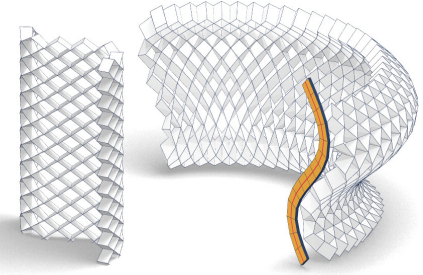
Fig. 10. Meshes deploying from a general profile (neither circle nor straight line) have rotational symmetry or are cylinders. This theoretical result is confirmed by these two examples which have been generated by optimization from C-mesh constraints, without prior knowledge of the global shape.
