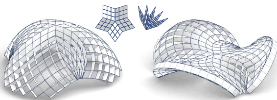
Fig. 21. These two examples of C-meshes with a combinatorial singularity correspond to surfaces which are tangent-continuous and piece-wise a K-surface (or offset of a K-surface). A combinatorial singularity never corresponds to a single piece of curvature-continuous surface. The small symbolic figure shows how such a mesh can deploy from a flat state after cutting it open.
