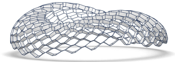
Fig. 14. A hexagonal C-mesh in the wider sense, exhibiting two different edge lengths. After cutting it becomes simply connected and collapses onto a circular strip.
