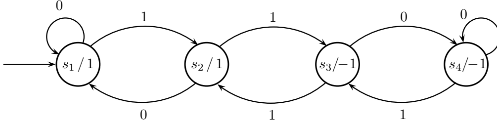
Figure 5.4: The Rudin-Shapiro sequence
