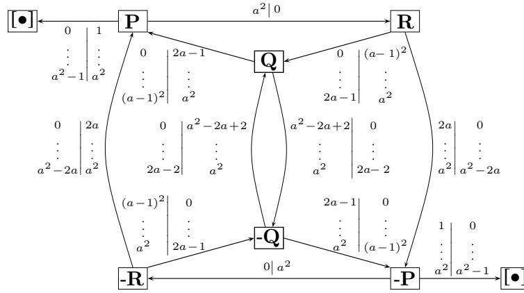
Figure 2.1: Addition automaton in base q = -a + i
