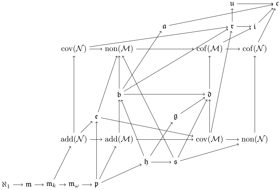
Figure 2. Cichoń’s diagram and the Blass diagram combined. An arrow \mathfrak{r} \rightarrow \mathfrak{h} means that ZFC proves \mathfrak{r} \leq \mathfrak{h} .
