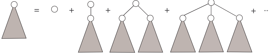
Fig. 1: Recursive structure of a planted plane tree
